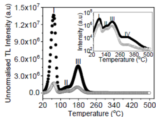
Figure 1. Thermoluminescence glow curves of natural quartz annealed at 1000 °C for 10 min (solid symbols) and 60 min (open symbols) measured at 1^\circ\text{C s}^{-1} following irradiation to 50Gy. The inset shows the same curves on a semilogarithmic plot which reveals the presence of peak IV.
